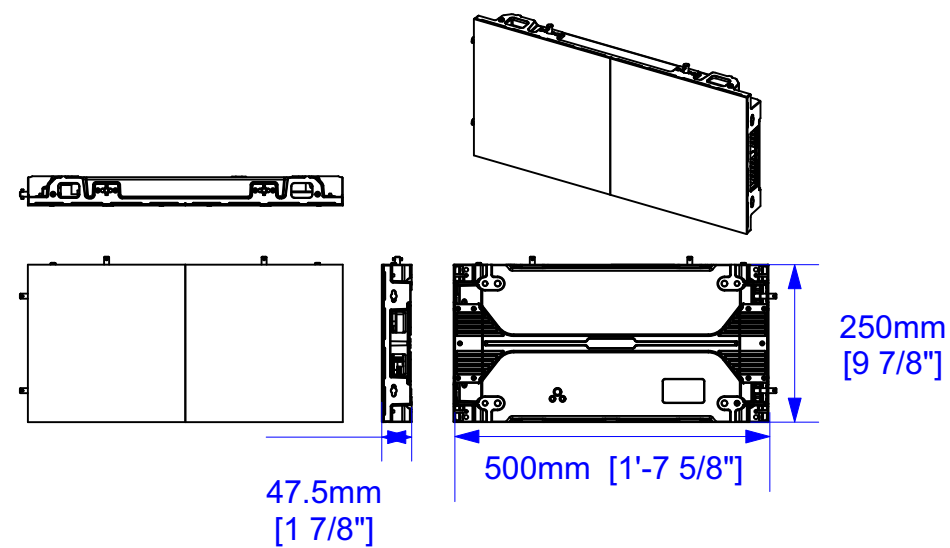
2 ATS PRO BRICK SERIES 500x250 Scale: 1:12
