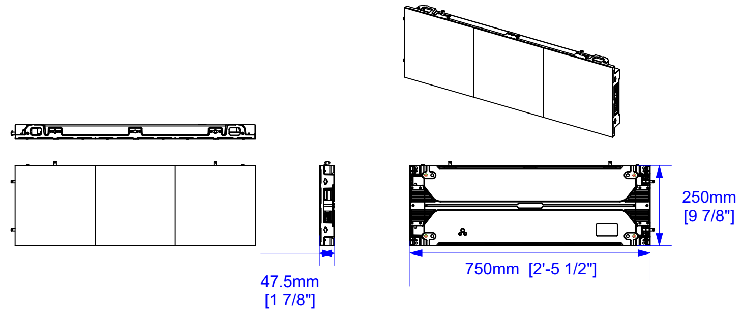
3 ATS PRO BRICK SERIES 750x250 Scale: 1:12
